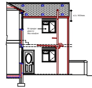
Proposed North East Elevation
