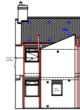
Proposed North West Elevation
