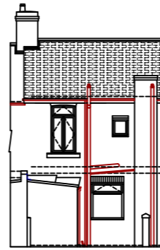
Existing North West Elevation
