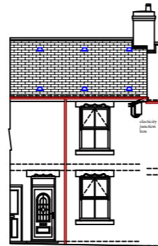
Proposed South East Elevation
