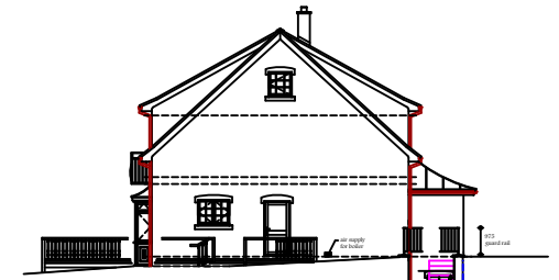
Proposed South West Elevation
