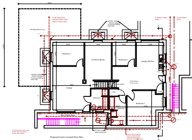
Proposed Lower Ground Floor Plan
