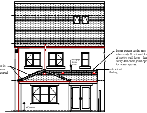
Proposed South Elevation
